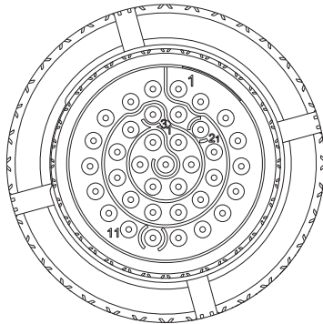
37P female Deutsch connector contact insertion view
