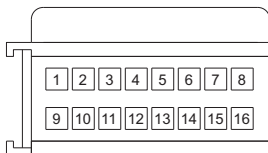
16P male AMP connector contact insertion view
