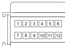
12P male AMP connector contact insertion view
