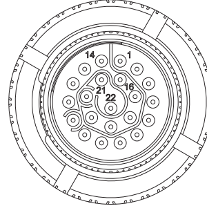
22P female Deutsch connector contact insertion view
